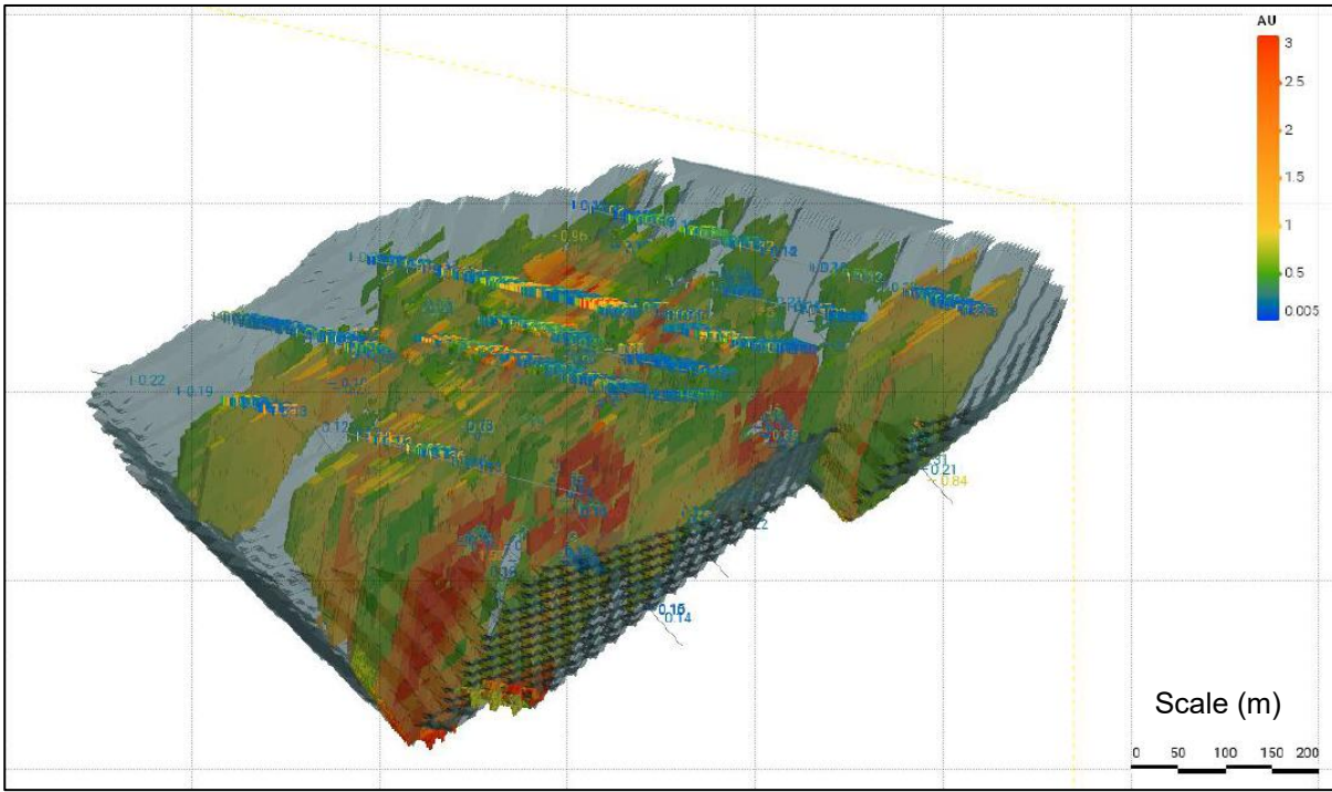
Figure 28. Oblique view of informing data and mineral domains block model for the MB01-S Inferred Mineral Resource Estimate and US$3,200/oz pit shell.
