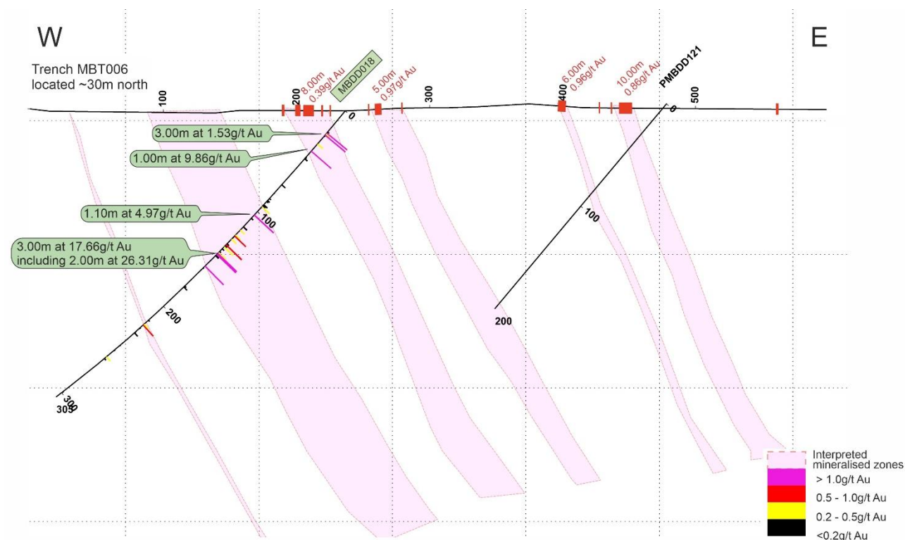
Figure 24. Interpretative cross section for fence line N872882 at MB01-S, with selected mineralised intervals from hole MBDD018 and planned hole location for PMBDD121 (note planned hole PMBDD212 was not drilled in Phase 1). See Figure 43 for an updated version including Phase 3 drilling results.
