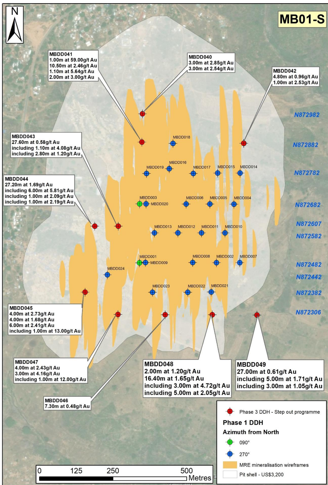
Figure 42. Plan view of MB01-S showing the Phase 3 Step-out programme drilling progress, selected best results from MBDD040 to MBDD049, drill collars from Phase 1 drilling and gold mineralised wireframes for the 870koz Au MRE within a US$3,200/oz pit shell.
