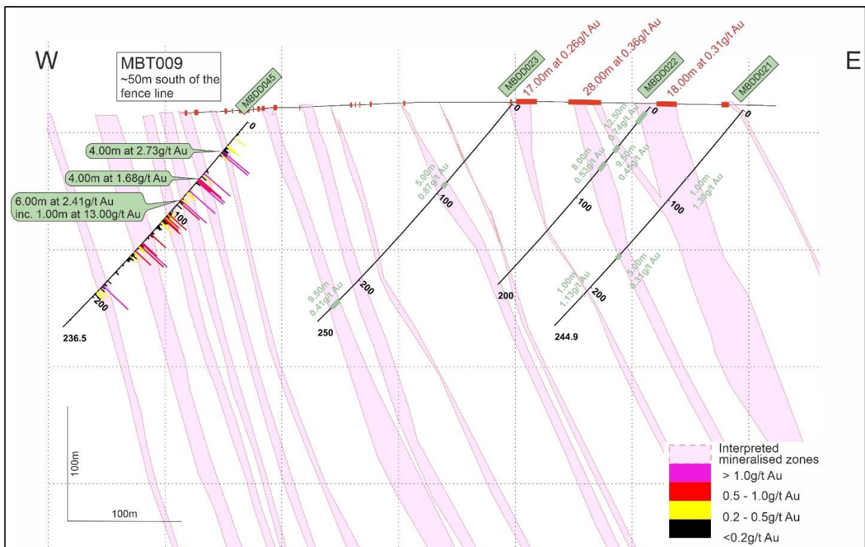
Figure 46. Simplified cross section of fence line N872382 with newly reported results from MBDD045. Previously reported best results from holes MBDD021 to MBDD023 and trench line MBT009 are also presented. MBT009 is located approximately 50m south of the fence line.
