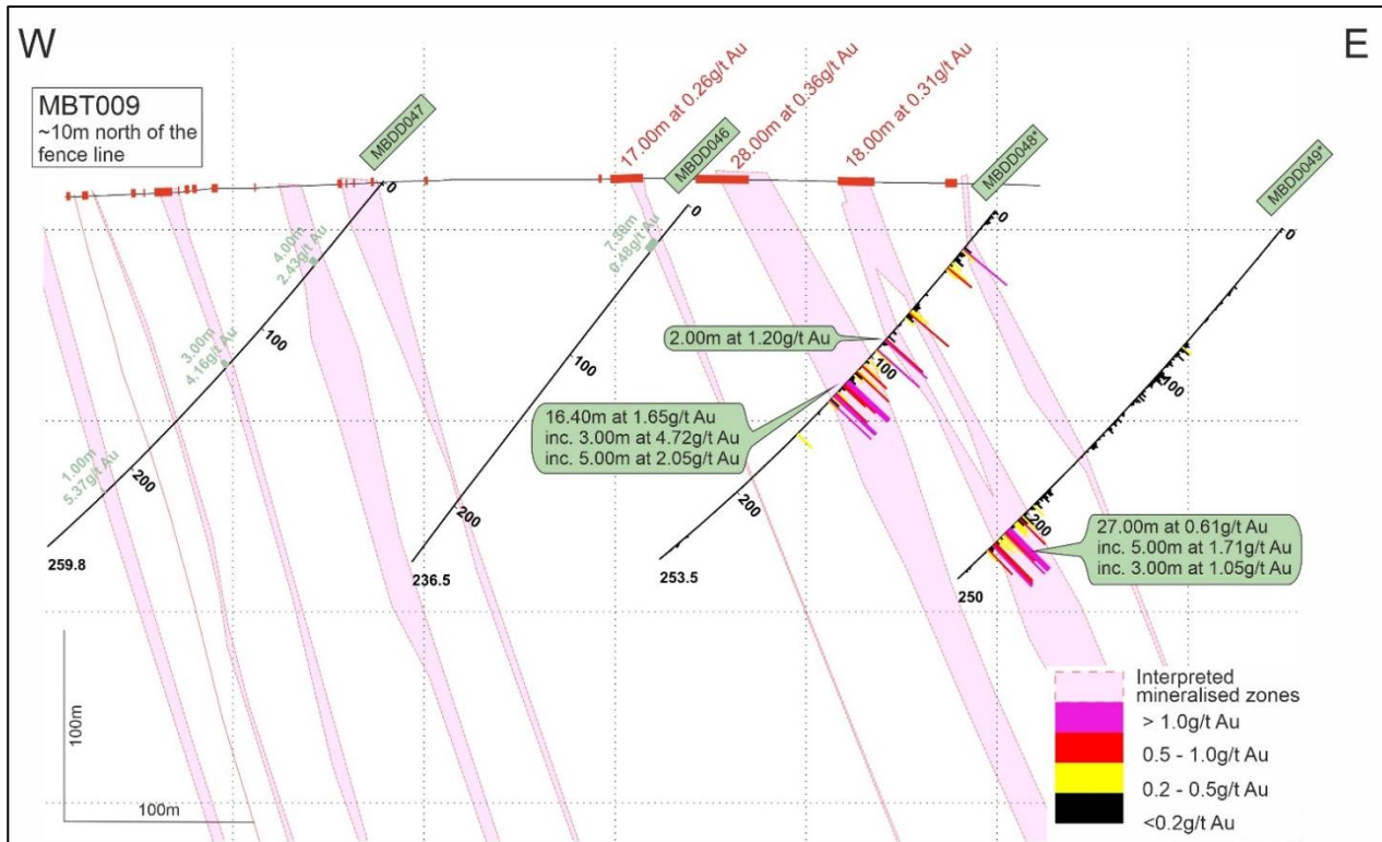
Figure 47. Simplified cross section of fence line N872306 with newly reported results from MBDD048 and MBDD049,. Previously reported best results from MBDD046, MBDD047, and trench line MBT009, located approximately 10m north of the fence line.
