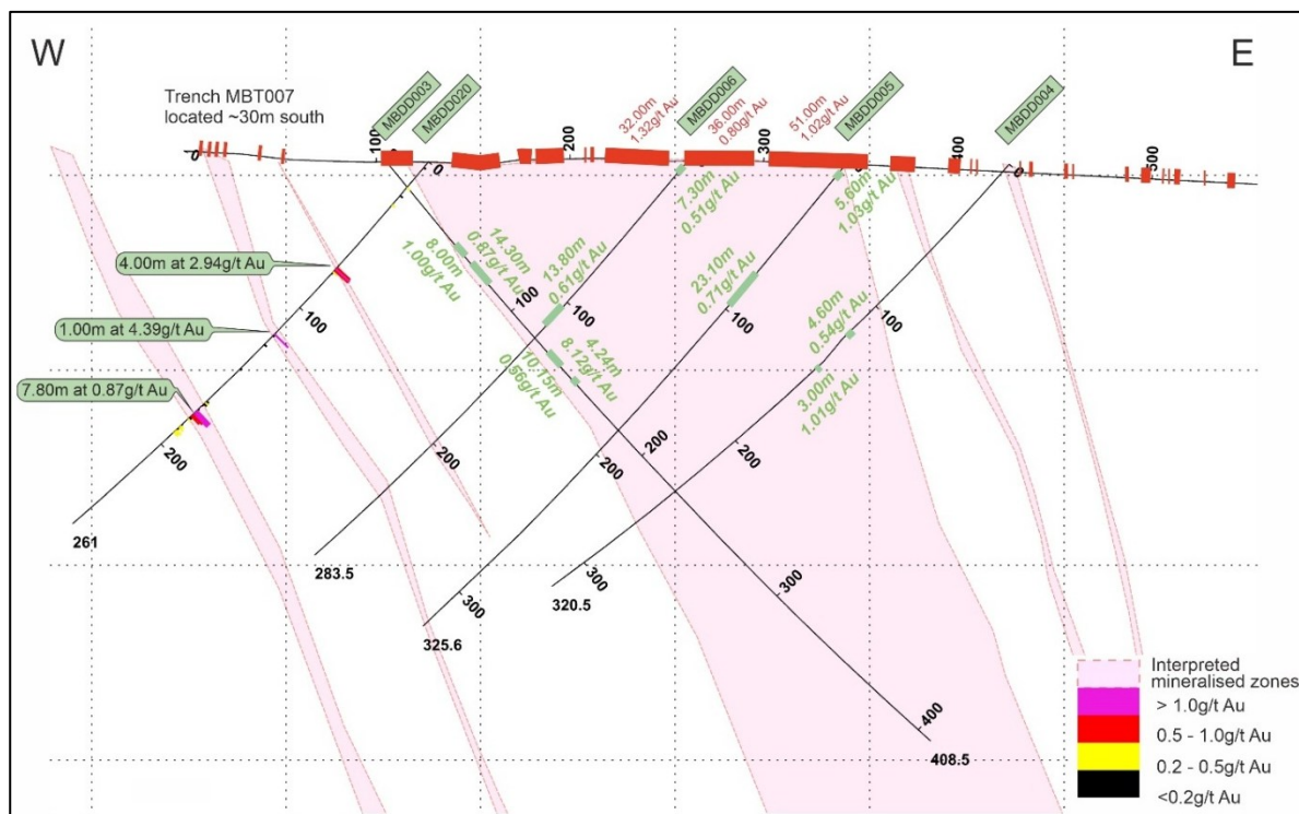
Figure 22. Interpretative cross section for fence line N872682 at MB01-S, with selected mineralised intervals from holes MBDD003 to MBDD006 and MBDD020. The fence line is located approximately 30m to the north of trench MBT007, the results for which are shown in red along the surface trace.
