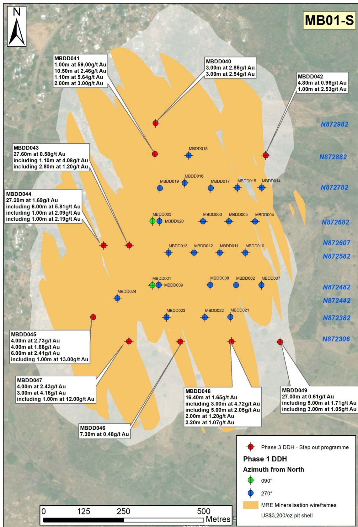
Figure 18. Plan view of MB01-S showing the Phase 3 Step-out collars with selected best results from MBDD040 to MBDD049, drill collars from Phase 1 drilling (MBDD001 to MBDD024) and gold mineralised wireframes for the 1.30Moz Au MRE within a US$3,200/oz pit shell.
