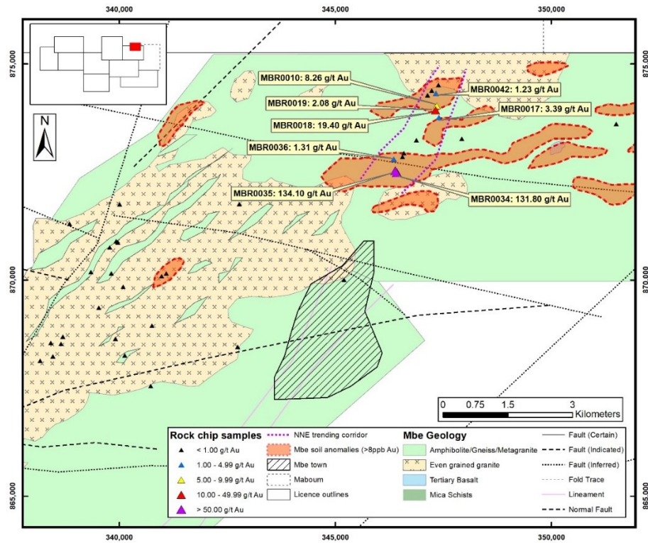
Figure 5. Mbe anomaly geological mapping (1:15,000) and rock-chip samples from selected outcrops within the Mbe anomaly area, predominantly focused on quartz veins that are hosted within a felsic porphyry unit that outcrops over a 3km-long north-northeast trending corridor.
