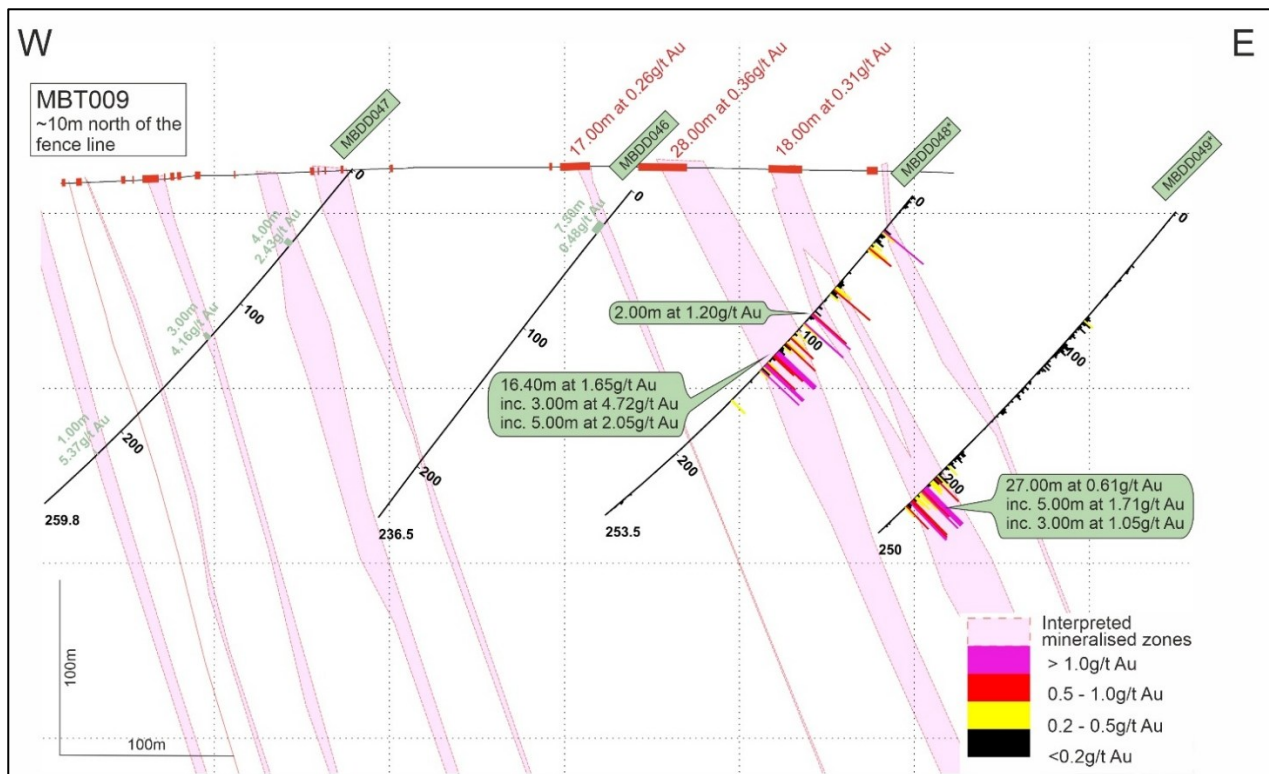
Figure 28. Simplified cross section of fence line N872306 with newly reported results from MBDD048 and MBDD049. Previously reported best results from MBDD046, MBDD047, and trench line MBT009, located approximately 10m north of the fence line.
