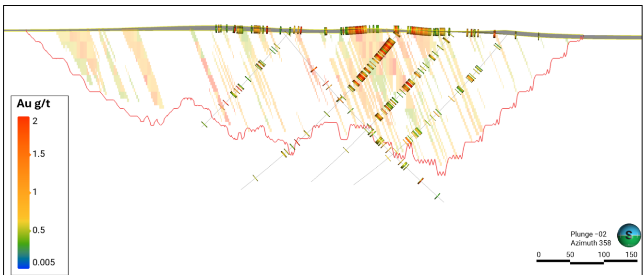
Figure 30. Cross section approximately along N872530 at MB01-S (viewing approximately north) showing the assay results from both trenching and drilling, the US$3,200/oz pit shell, and mineralised wireframe model.
