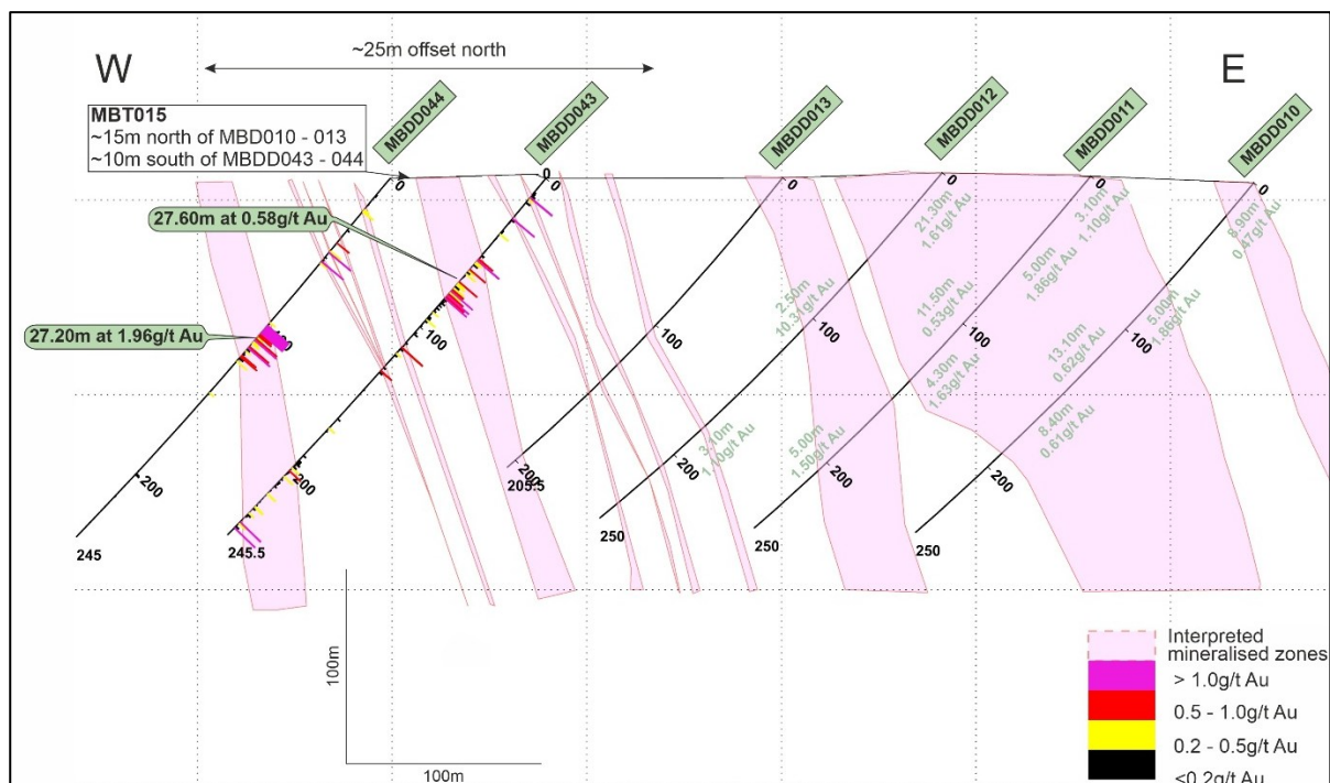
Figure 24. Simplified cross section of fence line N872582 with newly reported results from MBDD043 and MBDD044 (noting the ~25m offset to the north), previously reported best results from MBDD010 to MBDD013 and trench line MBT015 are also presented. MBT015 is located approximately 15m to the north of MBDD010 to MBDD013, and 10m to the south of MBDD043 and MBDD044.
