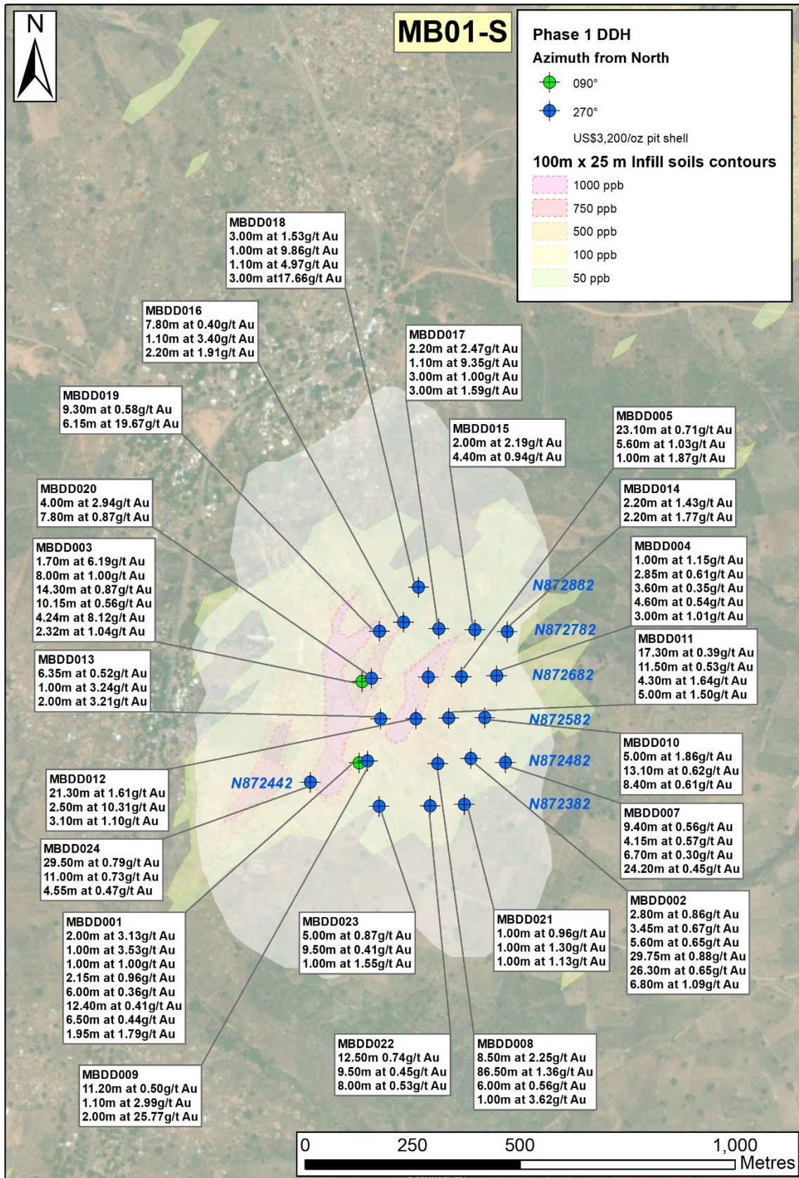
Figure 17. Plan for Phase 1 drilling at MB01-S with a selection of best results for each hole (MBDD001 to MBDD024) from fire assay analysis over gold-in-soil contours, and with the US$3,200/oz pit shell. Note the pit shell is defined from both Phase 1 and Phase 3 drilling, as well as Phase 1 and 2 trenching results.
