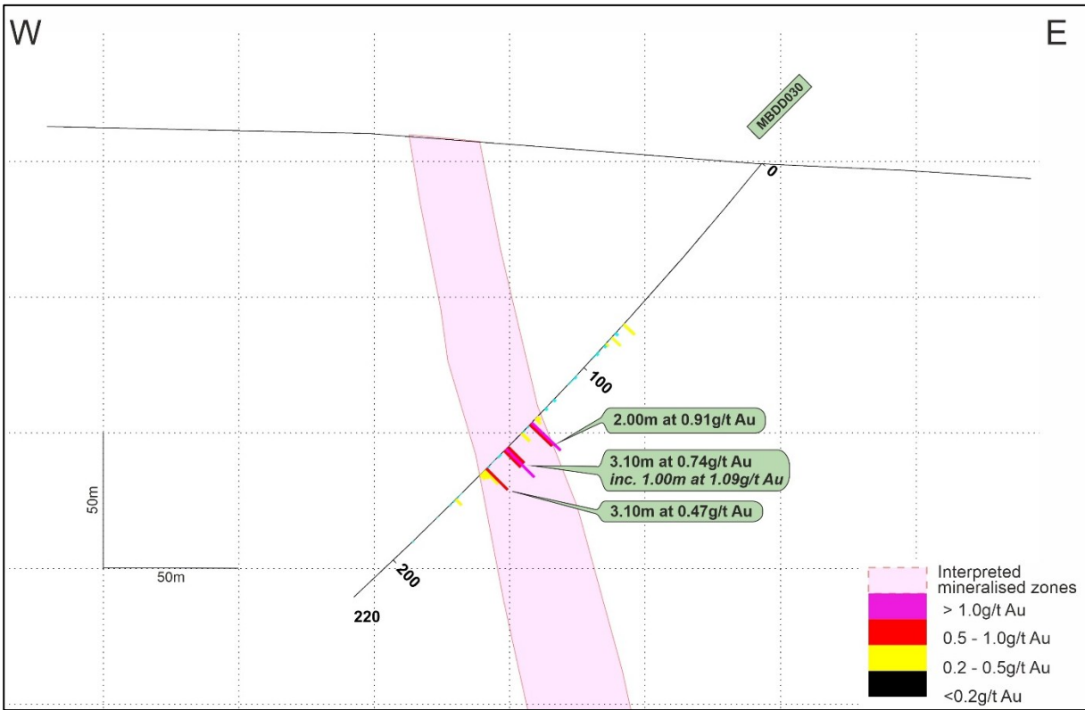
Figure 35. Simplified cross section for fence line N874025 with results from MBDD030 and interpreted mineralised zones.
