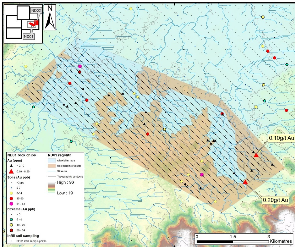
Figure 8. Rock chip sample results and infill soil sampling grid points (200m x 50m spacing) over interpreted regolith covering the ND01 area in central Ndom, with previous regional soil sampling results, and underlain by a Digital Elevation Model and generated streams.
