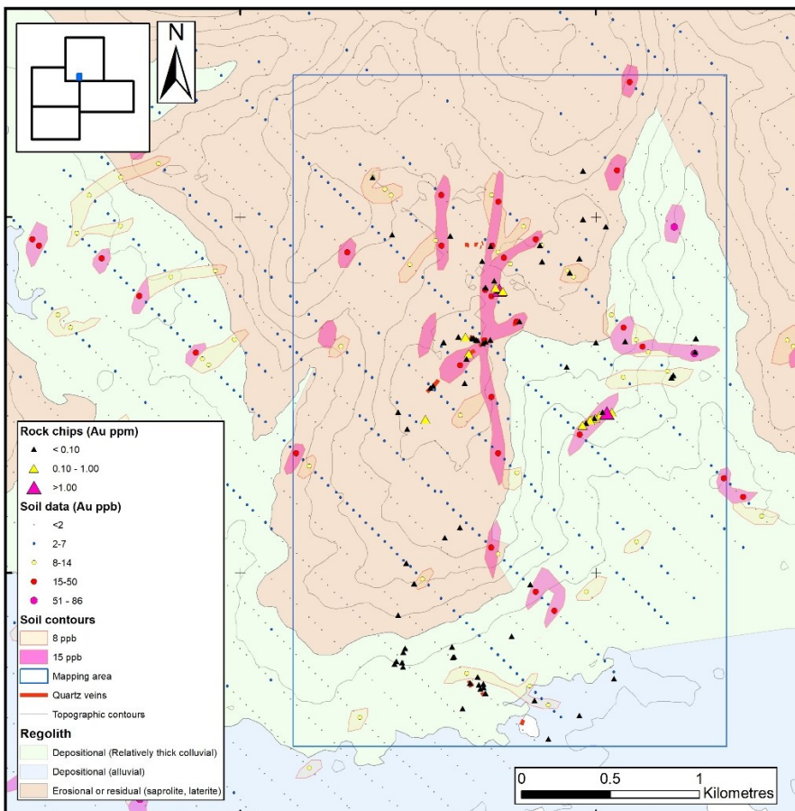
Figure 7. Rock-chip sampling results at PK01, on interpreted regolith map, infill soil sample data (200m x 50m) and Au contours, and area selected for more detailed geological mapping.
