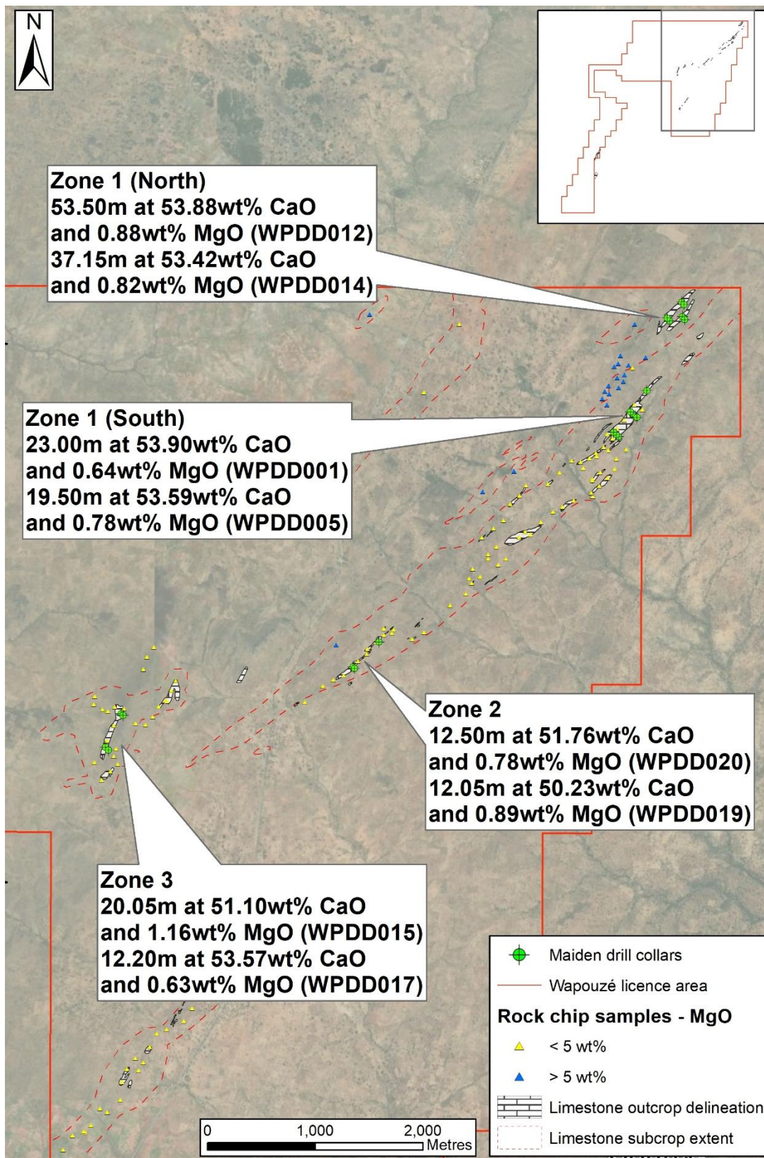
Figure 12. Wapouzé Programme drill plan showing the average chemistry from notable marble intervals. Plotted on MAXAR satellite image, and showing rock-chip sampling results with MgO values of less than 5wt% and more than 5wt% CaO shown in yellow. Samples with >50wt% CaO and <2wt% MgO are considered to have carbonate content suitable for use in the cement industry
